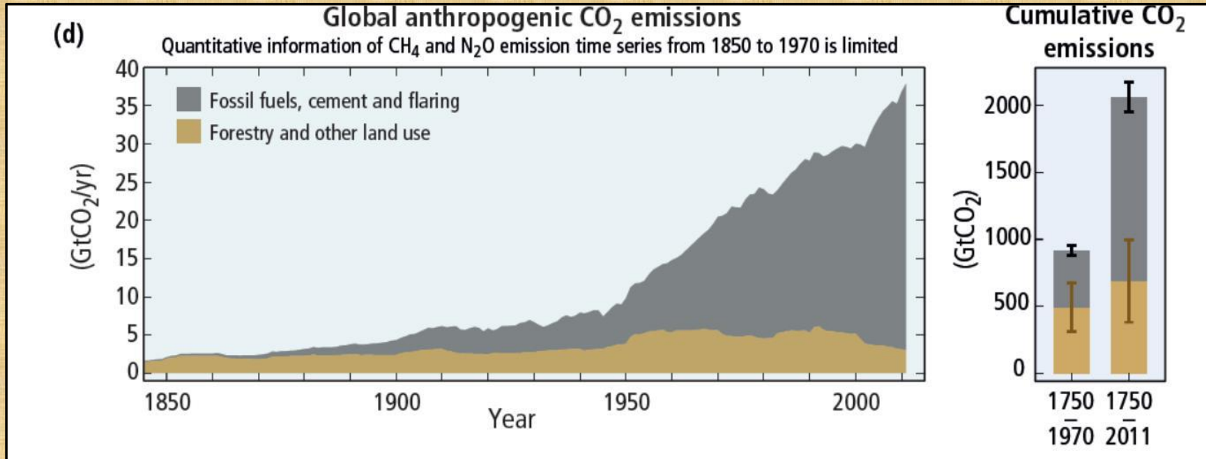
Figure: Global annual and cumulative greenhouse gas emissions at various dates
